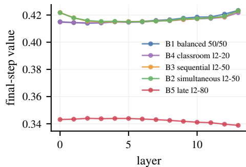
\kappa(W_{OV})
