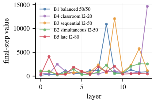
\kappa(W_{OV})
